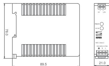
0165N-24V30W1AC
