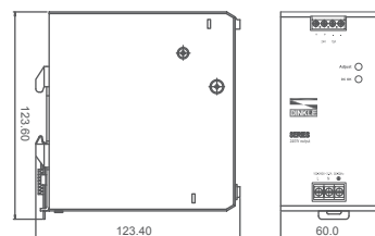
0165N-24V240W1AC
