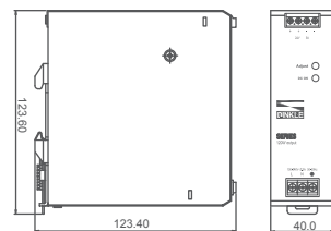
0165N-24V120W1AC
