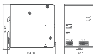
0165N-24V480W1AC
