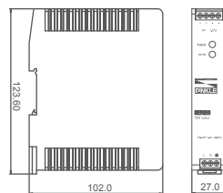
0165N-24V75W1AC
